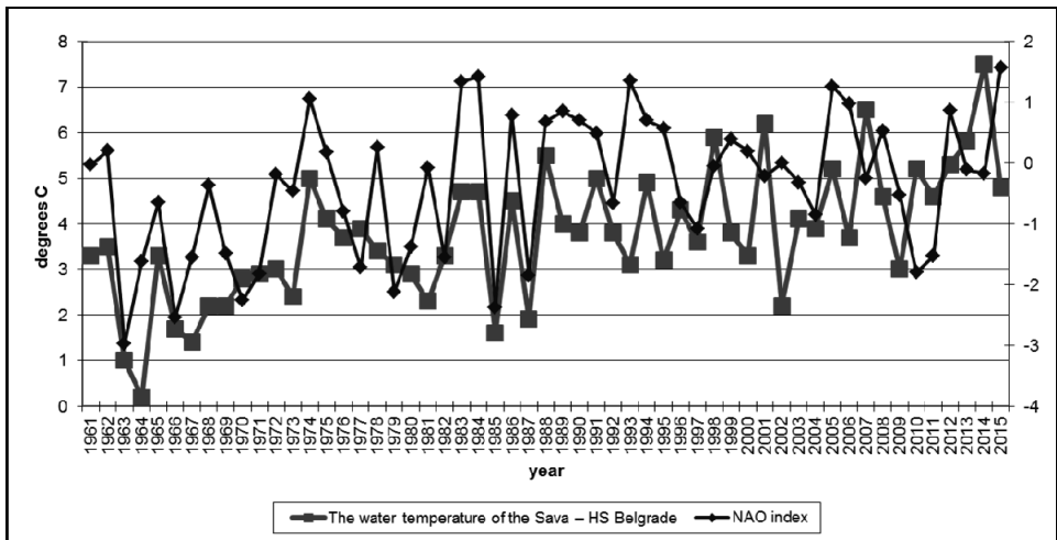
Figure 2. The water temperature of the Sava – HS Belgrade (January) and the NAO index January in the period 1961–2015: R=0.528 (significant at p \leq 0.01 )
