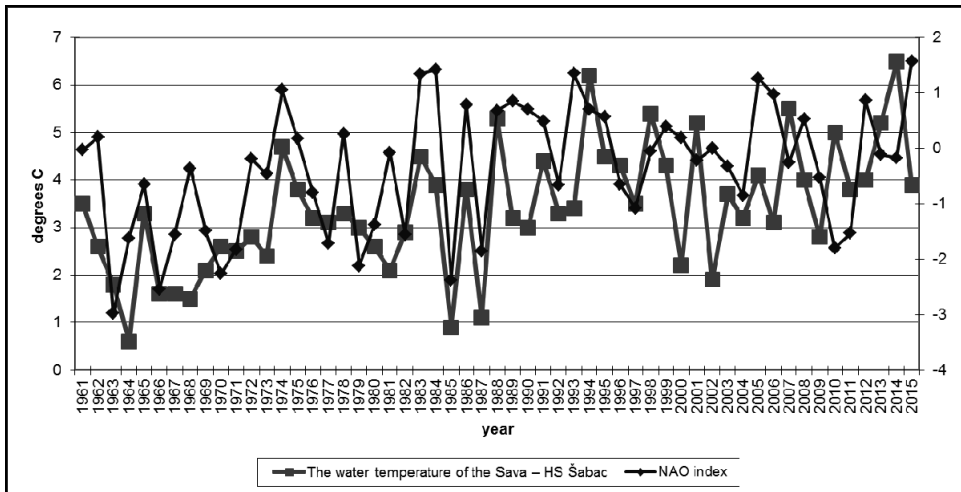
Figure 1. The water temperature of the Sava — HS Šabac (January) and the NAO index January in the period 1961–2015: R=0.512 (significant at p \leq 0.01 )
