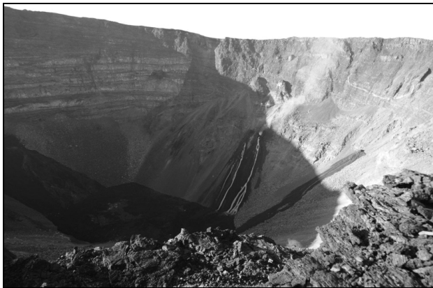
Figure 3a. Basalt lava erupts like fountain from aside cracks. Photo courtesy , Radovanović D.
